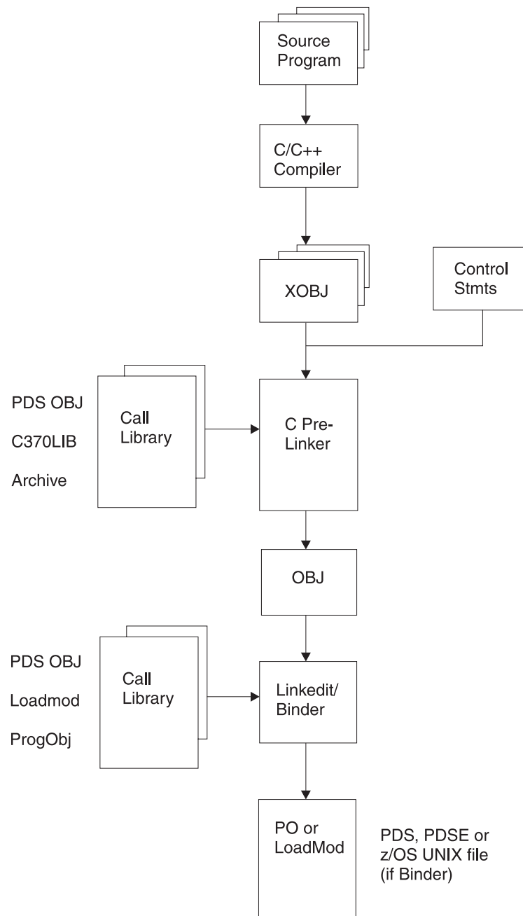
Figure 40. Invoking the prelinker. This diagram shows where the prelinker is invoked when the binder 'prelinker' function is not used.
