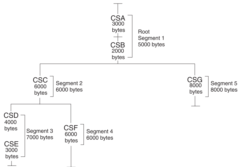
Figure 44. Length of an overlay module
