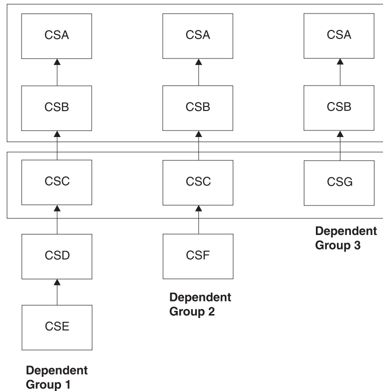
Figure 42. Control section dependencies
