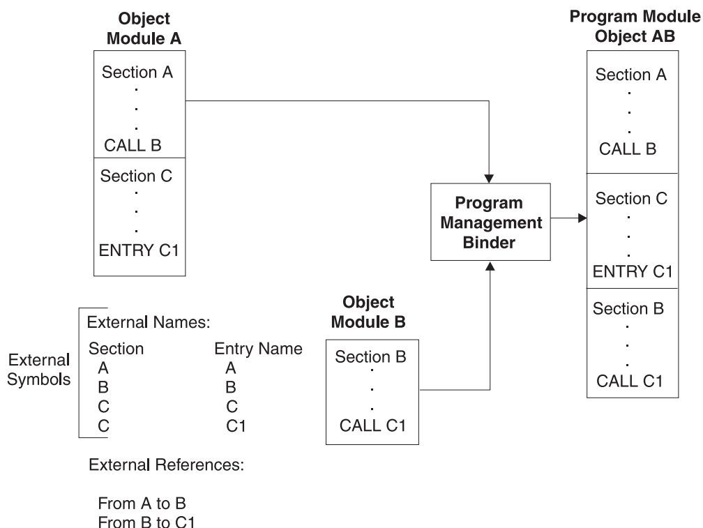
Figure 4. External names and external references
