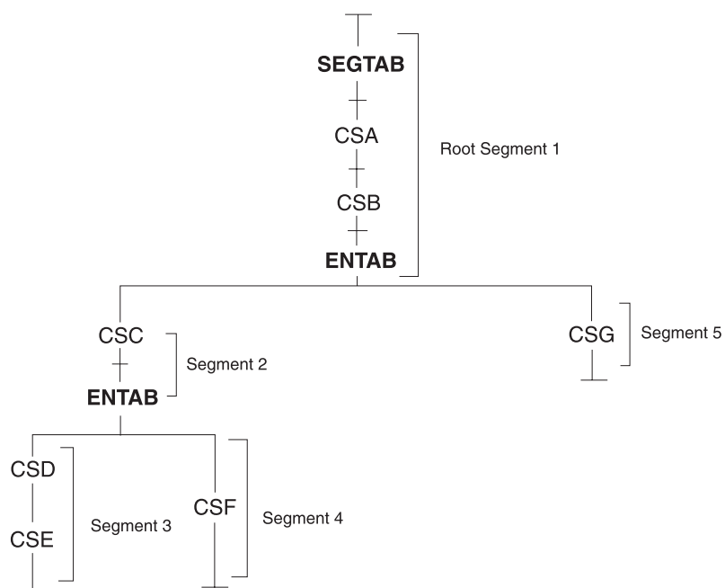
Figure 48. Location of segment and entry tables in an overlay module
