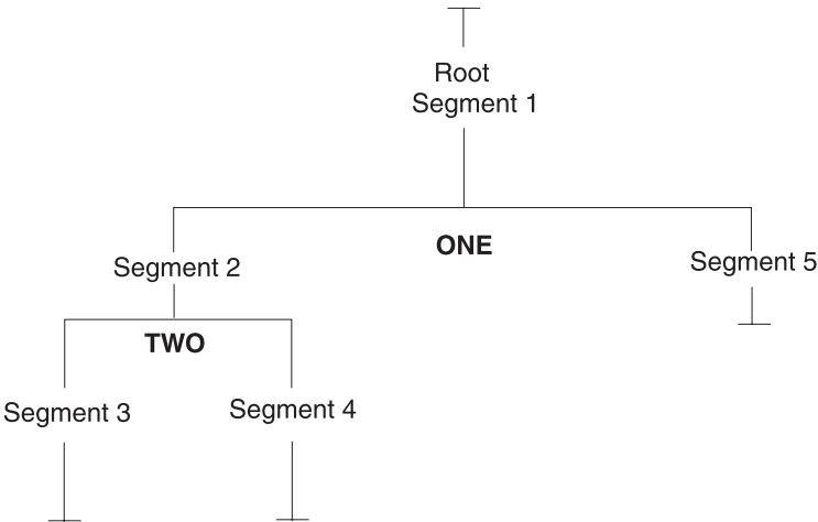
Figure 51. Symbolic segment origin in single-region program
