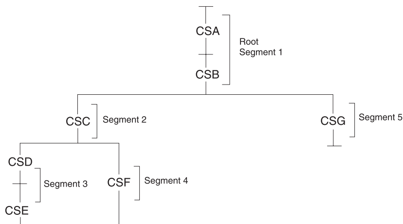
Figure 43. Single-region overlay tree structure
