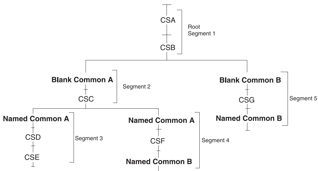
Figure 53. Common areas before processing
