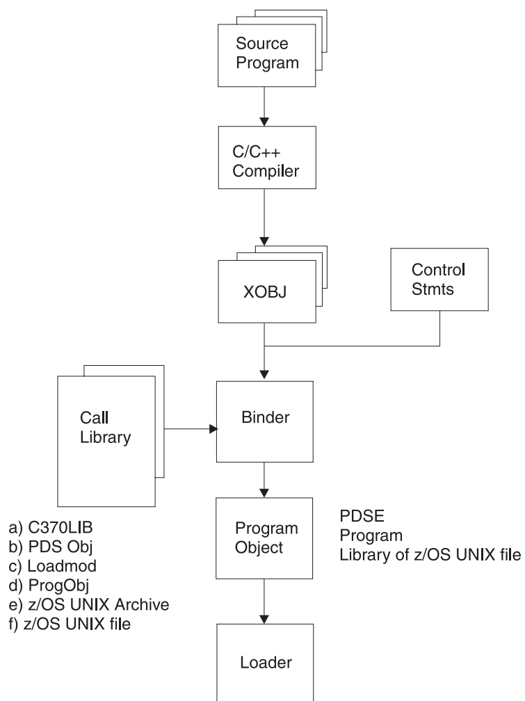
Figure 41. Prelinker elimination. This is the optional control flow in DFSMS/MVS 1.4.
