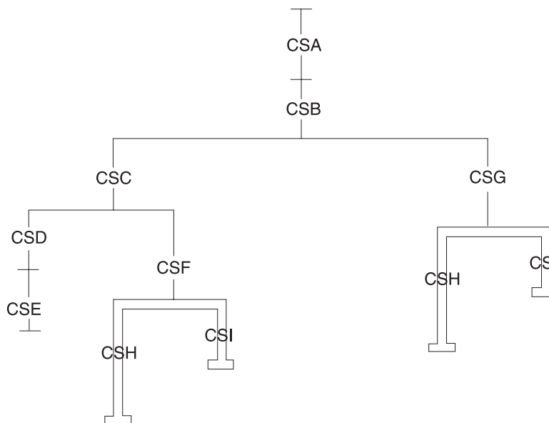
Figure 49. Control sections used by several paths
