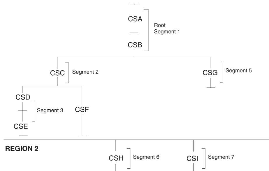
Figure 50. Overlay tree for multiple-region program
