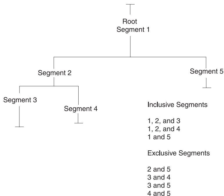
Figure 46. Inclusive and exclusive segments
