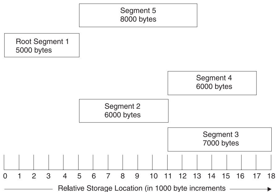
Figure 45. Segment origin and use of storage
