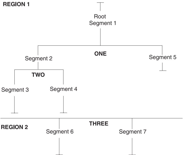
Figure 52. Symbolic segment and region origin in multiple-region program
