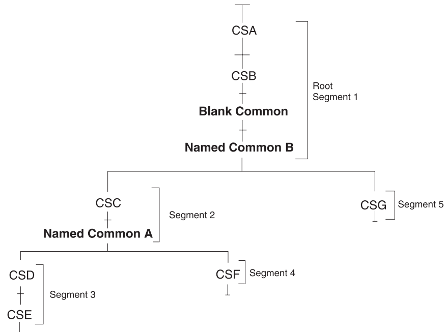
Figure 54. Common areas after processing
